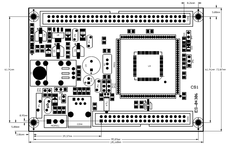
Figure 3: FLEX Light Base Board Dimensions
