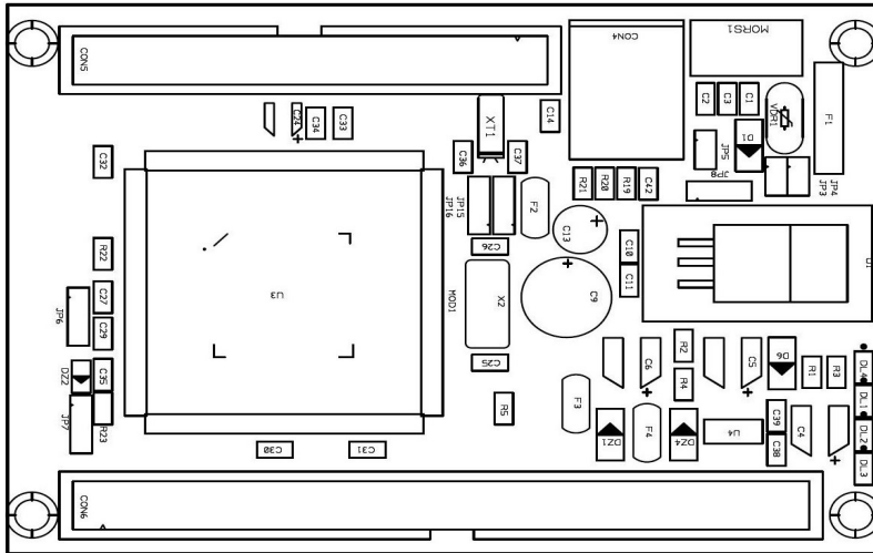
Figure 1: FLEX Light Base Board
