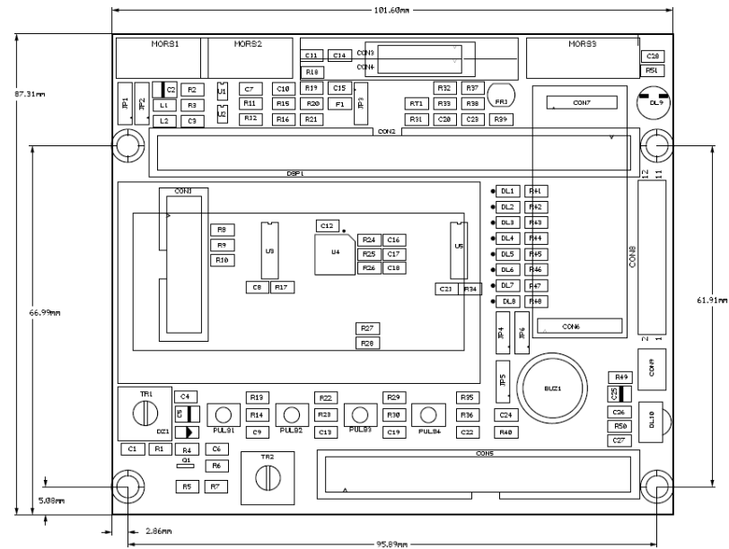
Figure 2: FLEX Demo Daughter Board Dimensions
