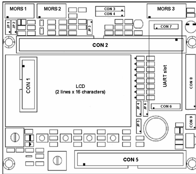
Figure 1: FLEX Demo Daughter Board
